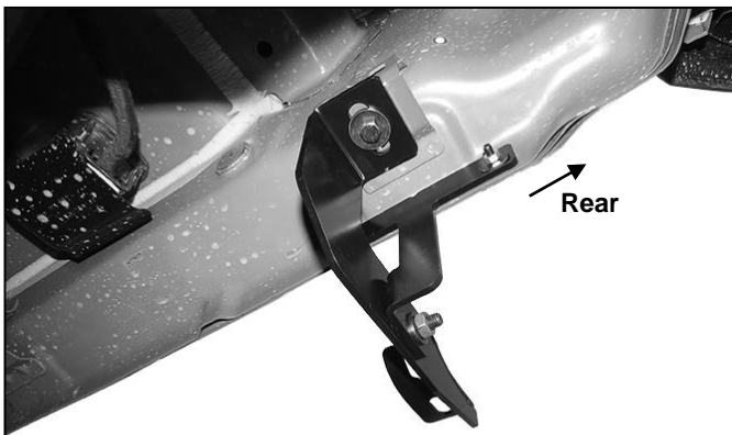
(Fig 12) Passenger/Right Center Mounting Bracket and Support Bracket attached to 2nd location
