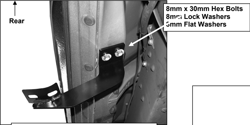
(Fig 5) Driver/Left Rear Bracket installed
