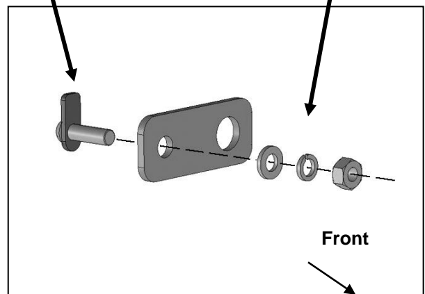
(Fig 13) Attach sensor to Relocation Bracket. Attach Bracket to Bolt Plate (fig 11)
