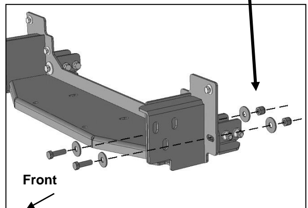
(Fig 18) Attach the Winch Tray assembly to the Support Brackets
