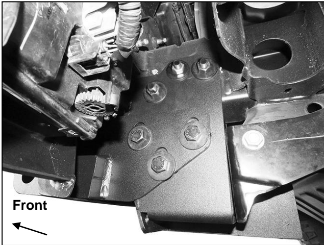
(Fig 23) Driver/left side of CS1 Bumper attached to Frame Bracket (Note OEM light installation)
