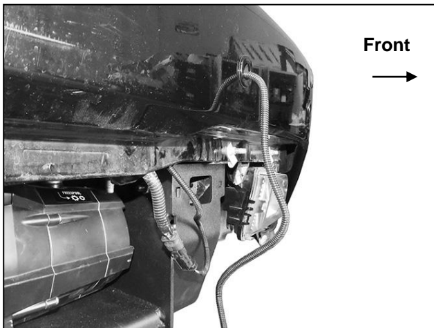
(Fig 21) Reinstall factory bumper. Models with sensors, plug Wire Harness Extensions into the sensors in the CS1 HD Bumper
