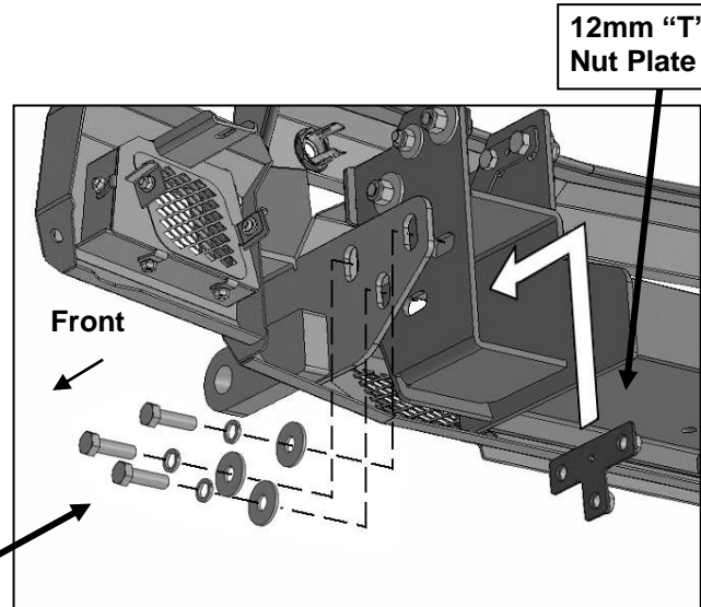
(Fig 22) Insert "T" Nut Plates into back of Frame Brackets. Attach CS1 Bumper to outside of Frame Brackets and to Nut Plates.
