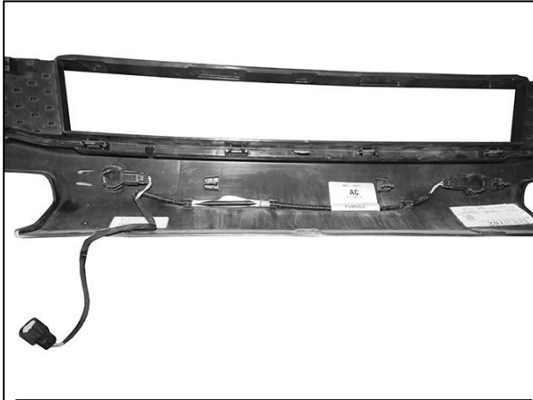
(Fig 15) Models with sensors, remove sensors and harness from plastic panel
