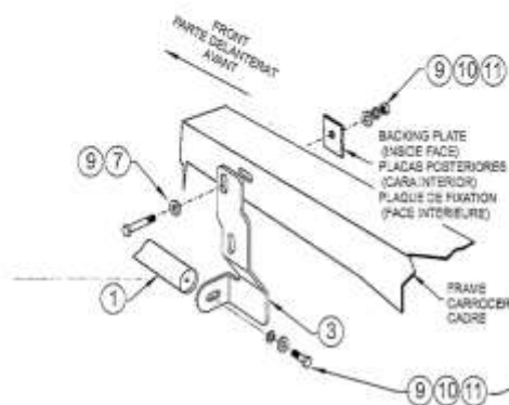
FIGURE 2 INSTALLATION VIEW OF DRIVER SIDE SHOWN FIGURA 2 VISTA DE LA INSTALACIÓN DEL LADO DEL CONDUCTOR FIGURE 2 ILLUSTRÉ: CÔTE CONDUCTEUR
