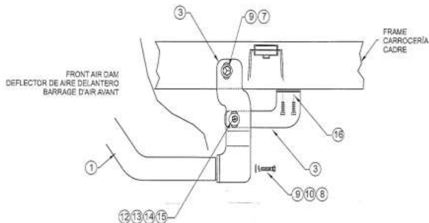
FIGURE 1 INSTALLATION VIEW OF DRIVER SIDE SHOWN FIGURA 1 VISTA DE LA INSTALACIÓN DEL LADO DEL CONDUCTOR FIGURE 1 ILLUSTRÉ: CÔTE CONDUCTEUR
