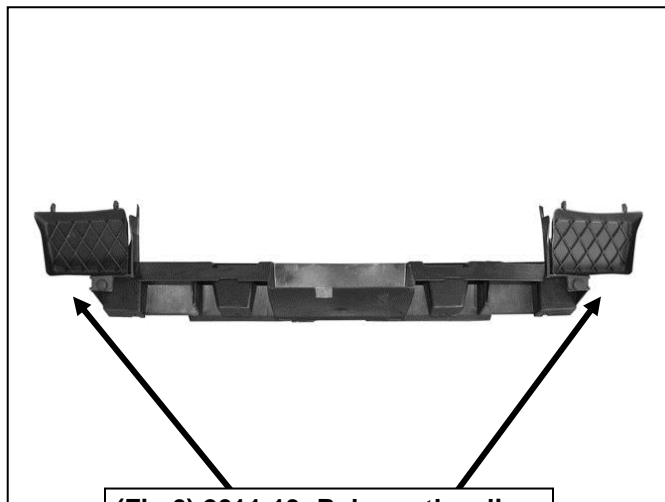
(Fig 6) 2011-13: Release the clips to remove both air block offs
