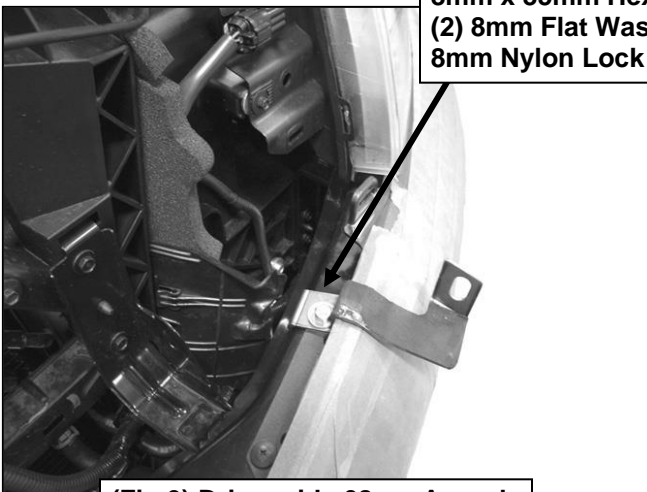
(Fig 9) Driver side 08-up Armada Top Bracket pictured
