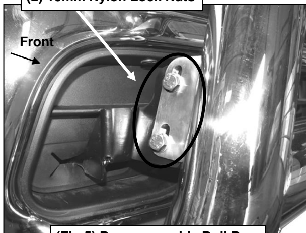
(Fig 5) Passenger side Bull Bar Bracket attached to Bull Bar
