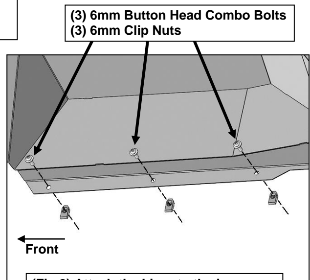
(Fig 2) Attach the Liner to the inner body panel. (NOTE: Slide the (3) Clip Nuts onto the panel first)
