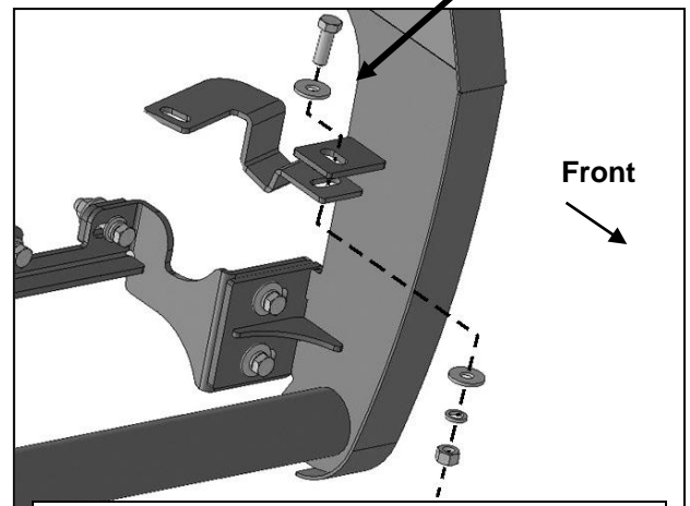
(Fig 18) driver side 2013-16 Upper Bracket
