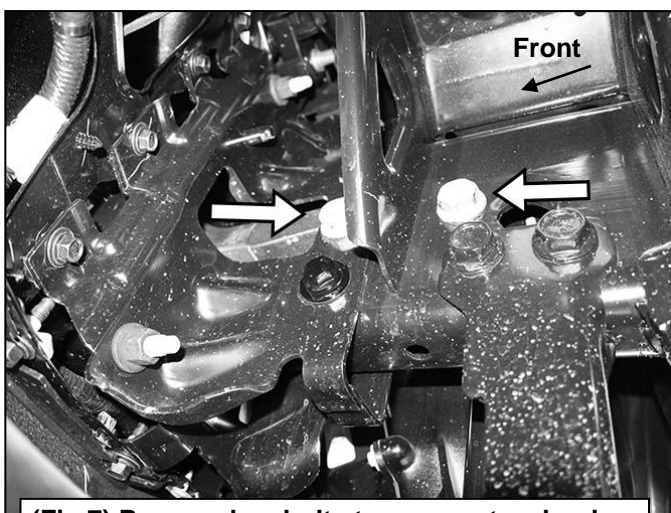
(Fig 7) Remove hex bolts to remove tow hook
