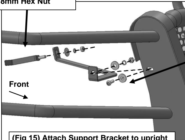
(Fig 15) Attach Support Bracket to upright (For Example Only)
