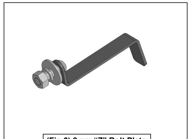
(Fig 6) 8mm "Z" Bolt Plate
