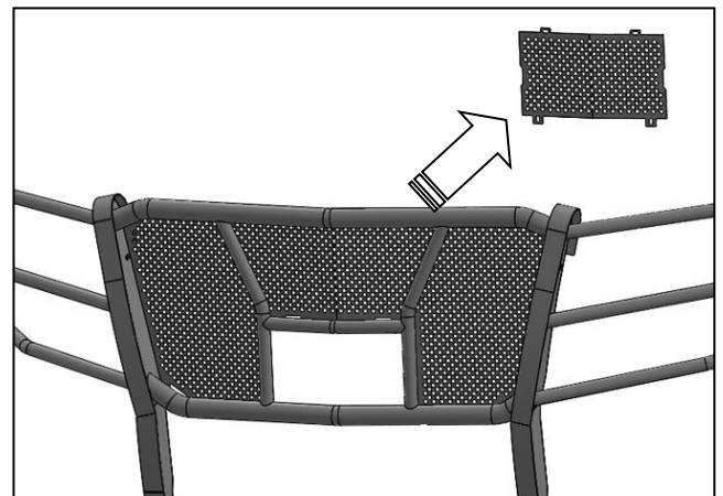
(Fig 16) Remove screen from grille for models with grille mounted camera (For Example Only)
