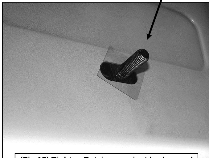
(Fig 15) Tighten Retainer against body panel
