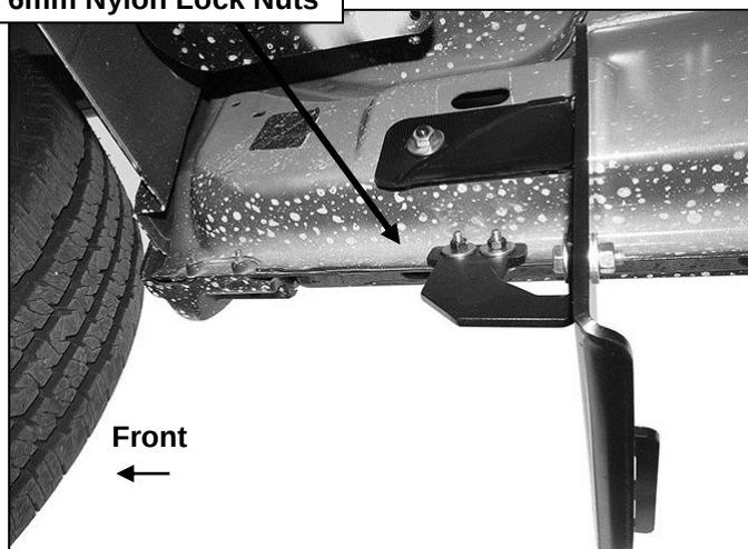
(Fig 13) Passenger side front Bracket assembly
