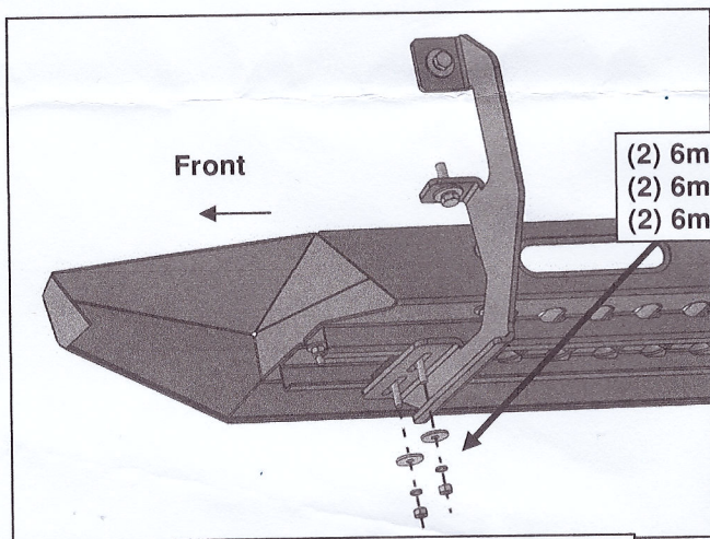
(Fig 11) Front of Running Board attached to Mounting Bracket
