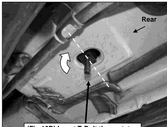
(Fig 16B) Insert T-Bolt then rotate 90-degrees to go across oval hole
