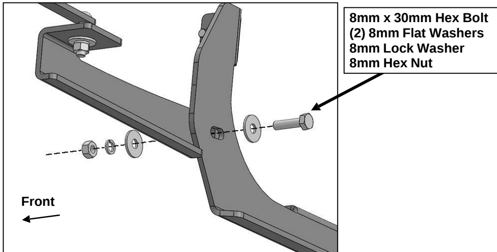
(Fig 6) Attach Passenger/Right Front Support Bracket to Mounting Bracket
