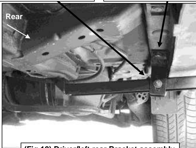
(Fig 12) Driver/left rear Bracket assembly
