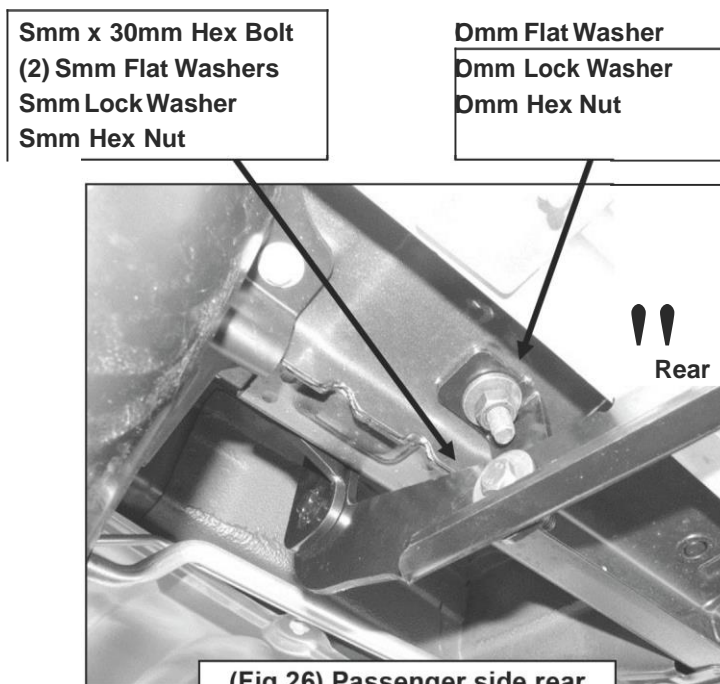
(Fig 26) Passenger side rear Bracket pictured from below
