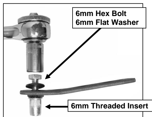
(Fig 2) 6mm Threaded Insert Tool assembly pictured
