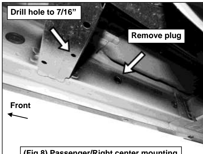
(Fig 8) Passenger/Right center mounting location. If necessary, drill out small hole to 7/16\"
