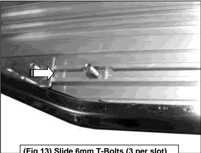
(Fig 13) Slide 6mm T-Bolts (3 per slot) into slots on bottom of Running Board
