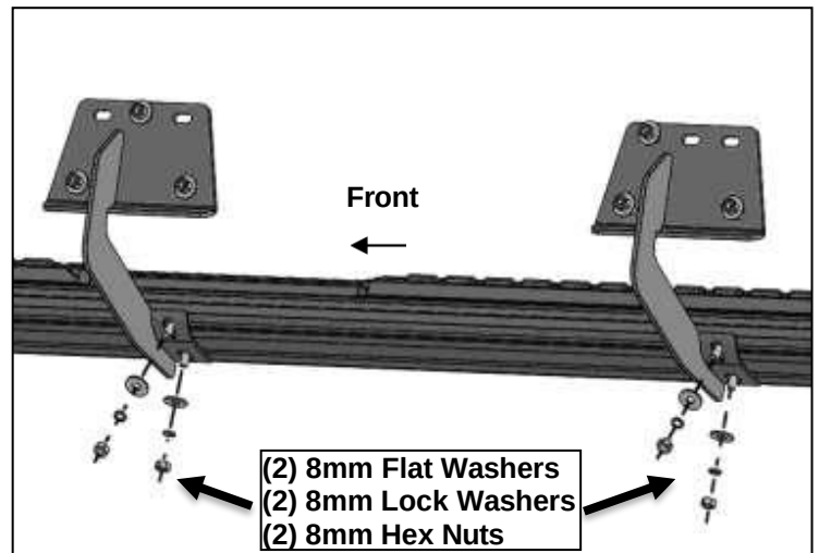
(Fig 11) Passenger/right Sidebar attached to mounting brackets at the center and rear locations.
