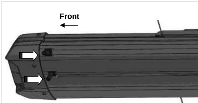
(Fig 9) Insert 8mm Hex-Bolts through the channel openings in the bottom of the sidebar.
