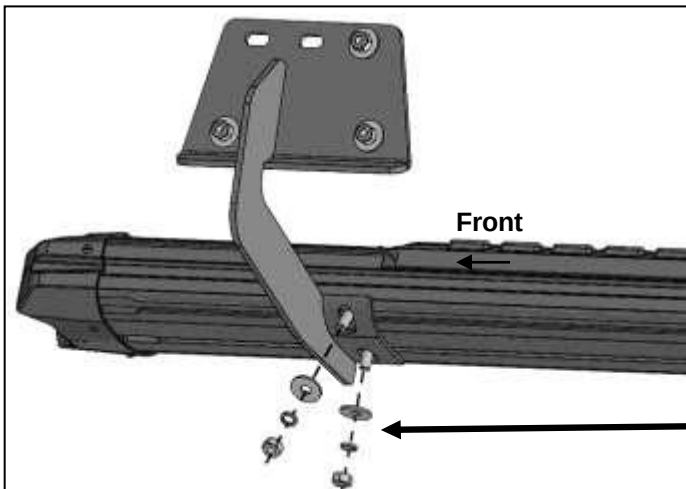
(Fig 10) Passenger/right Sidebar attached to Mounting Bracket at the front location.
