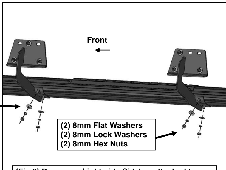
(Fig 8) Passenger/right side Sidebar attached to Mounting Brackets at the center and rear locations
