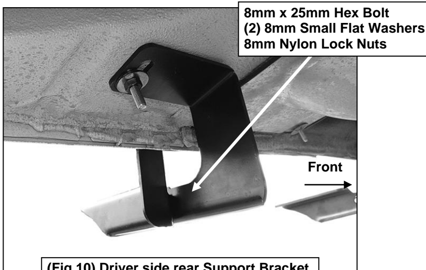
(Fig 10) Driver side rear Support Bracket
