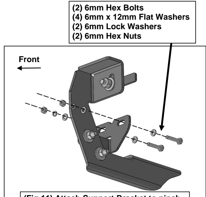
(Fig 11) Attach Support Bracket to pinch weld (passenger front Bracket illustrated)
