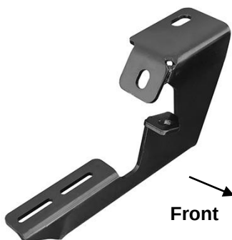
(Fig 17) Passenger side #2 Bracket
