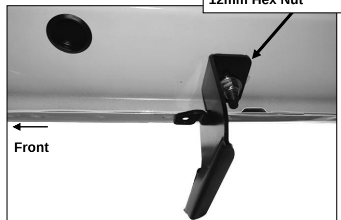
(Fig 21) Passenger side #3 Mounting Bracket
