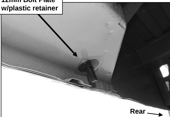
(Fig 22) Passenger/right rear mounting location
