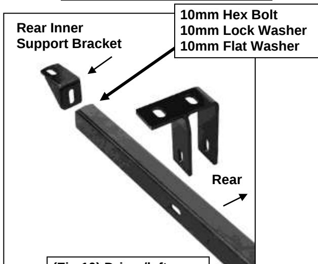
(Fig 10) Driver/left rear Bracket assembly
