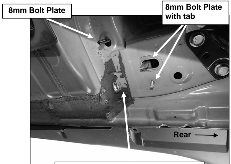
(Fig 6C) Passenger rear mounting location pictured from below. Scrape off excess sealant from mounting location before installing rear Bracket
