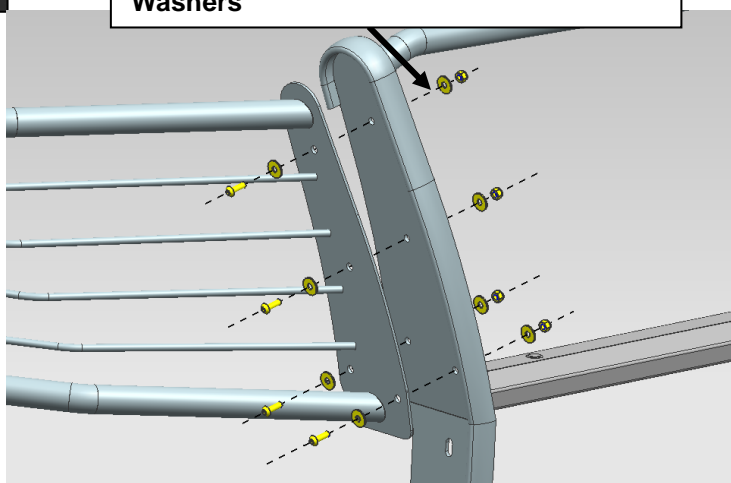
(Fig 12) Attach Right Brush Board to Middle Guard.
