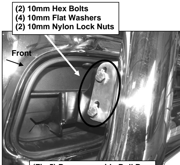
(Fig 5) Passenger side Bull Bar Bracket attached to Bull Bar
