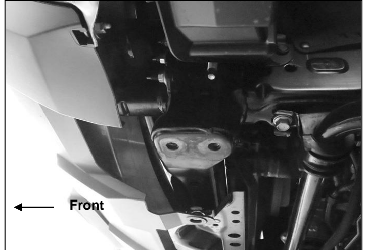
(Fig 2) Driver side tow hook mounting location
