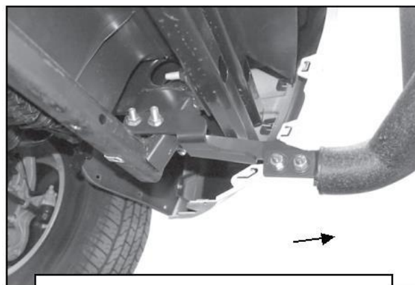
(Fig 14) driver/left complete installation
