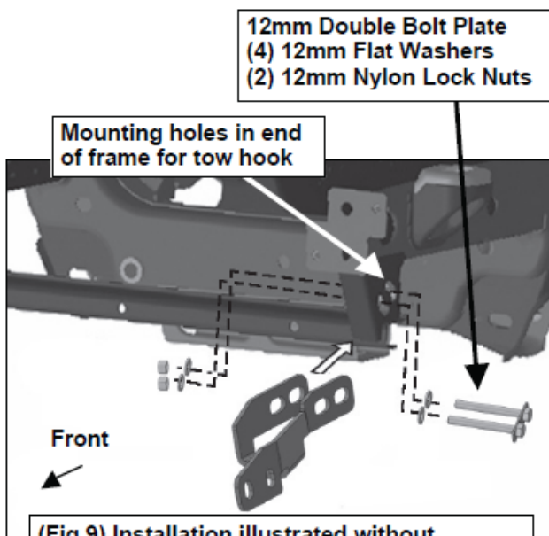
(Fig 9) Installation illustrated without bumper cover for instruction purposes only. Do not remove bumper cover.
