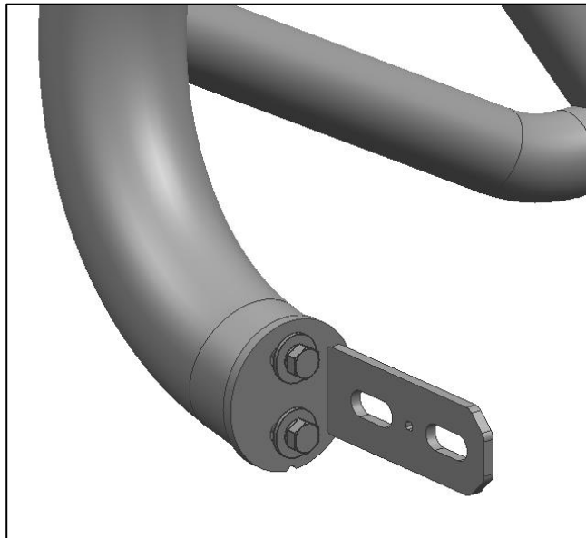
(Fig 12) left/driver side Tube Bracket to Guard
