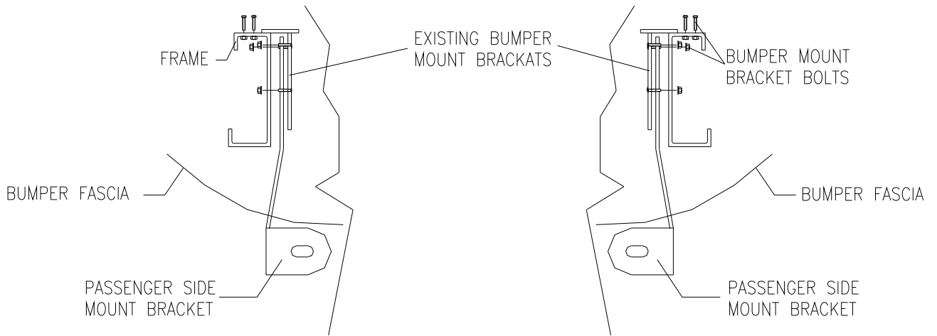
FIGURE 1 FRONT VIEW
