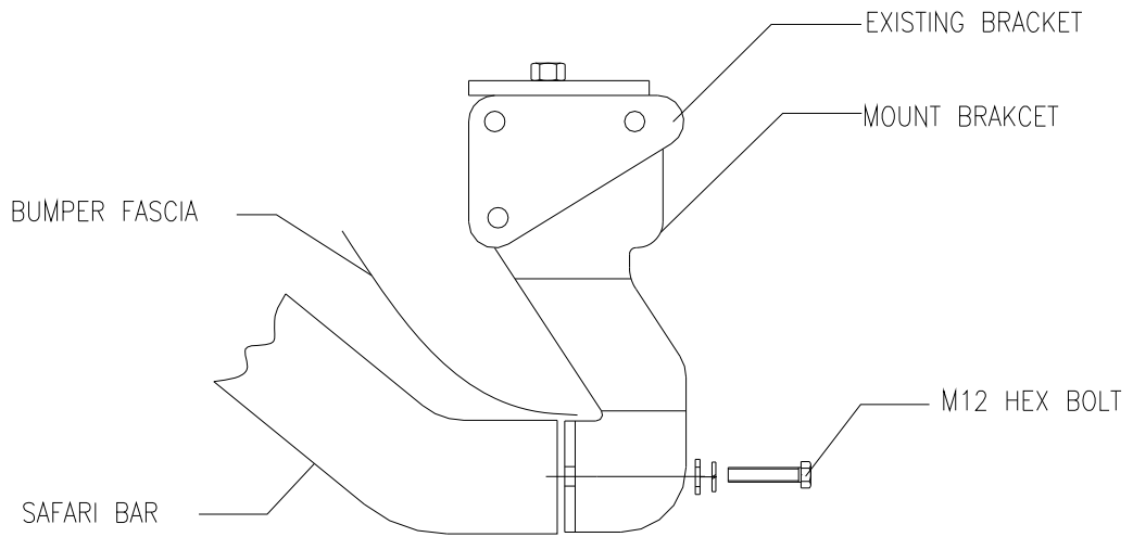
FIGURE 2 DRIVER SIDE
