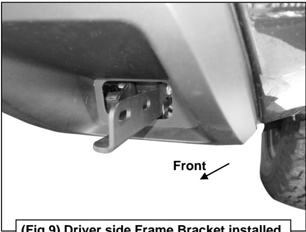
(Fig 9) Driver side Frame Bracket installed
