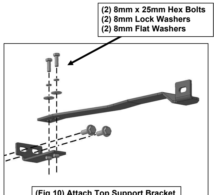
(Fig 10) Attach Top Support Bracket to top of Mounting Bracket
