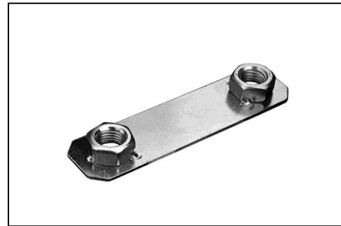
(Fig 9) Models without tow hooks, insert 12mm Double Nut Plates into end of frame (see Fig 8)
