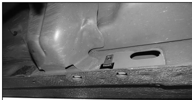
(Fig 4) Passenger/right front or rear Bracket attached to pinch weld
