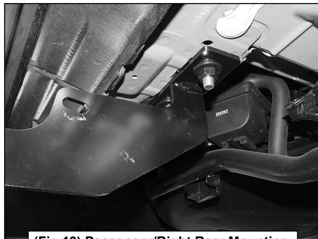
(Fig 13) Passenger/Right Rear Mounting Bracket attached to the (2) Bolt Plates
