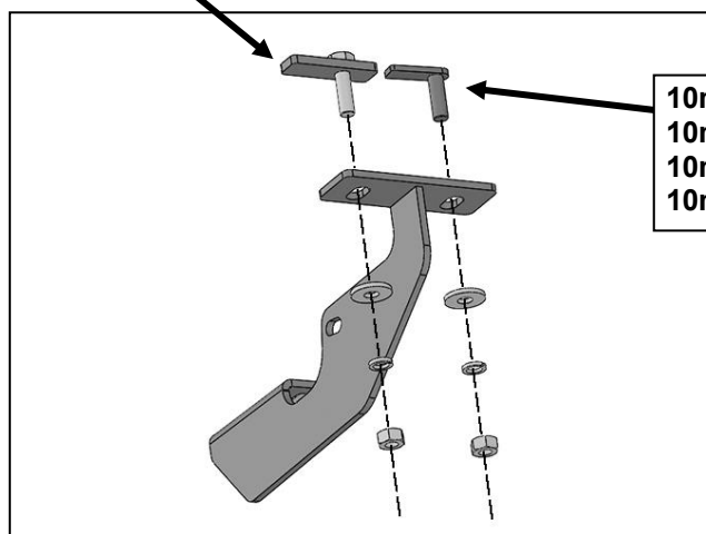
(Fig 12) Attach the Passenger/Right Rear Mounting Bracket to the inner (1) 10mm Small Bolt Plate and the 10mm Large Bolt Plate
