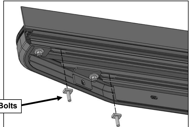
(Fig 17) Insert (6) 6mm T-Bolts into the bottom of the Running Board, (3) per channel
