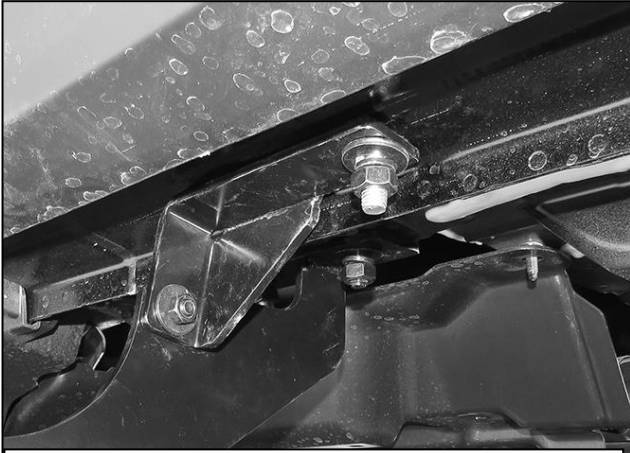
(Fig 16) Passenger/Right Rear Support Bracket attached to the Mounting Bracket and vehicle
