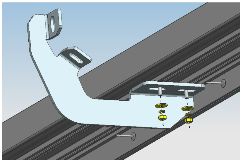
(Fig 6) Attach the Passenger/Right Running Board to the Mounting Brackets
